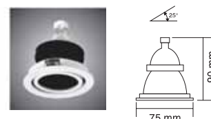
SP-MR16-3 MAX QR-CB51 50W 12V GU5.3
