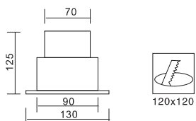
MUM-5121 MR16 50W GU5.3
