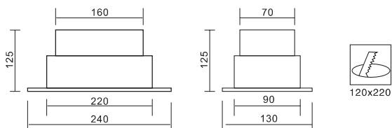
MUM-5122 MR16 50Wx2 GU5.3
