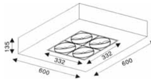
MUC-03R QR111 Max 50Wx4 G53 TC-L 36Wx4 2G11
