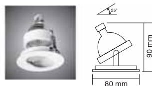
SP-MR16-2 MAX QR-CB51 50W 12V GU5.3
