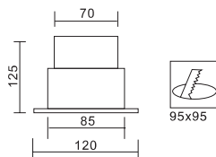
MUM-5111 MR16 50W GU5.3
