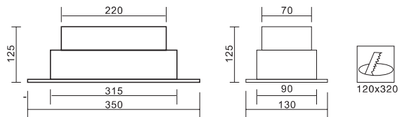
MUM-5133 MR16 50Wx3 GU5.3
