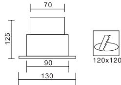
MUM-5131 MR16 50W GU5.3
