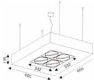
MUC-03P QR111 Max 50W x4 G53 TC-L 36Wx4 2G11
