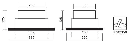
MUA-5022 QR111 50Wx2 G53
