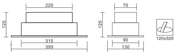
MUM-5123 MR16 50Wx3 GU5.3
