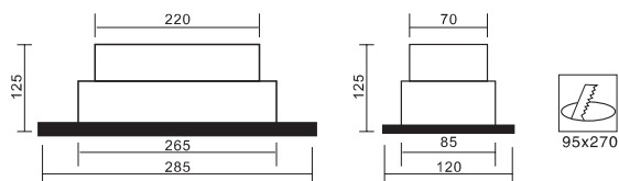
MUM-5113 MR16 50Wx3 GU5.3
