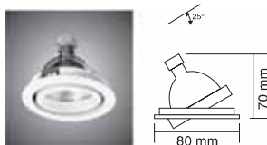
SP-MR16-1 MAX QR-CB51 50W 12V GU5.3
